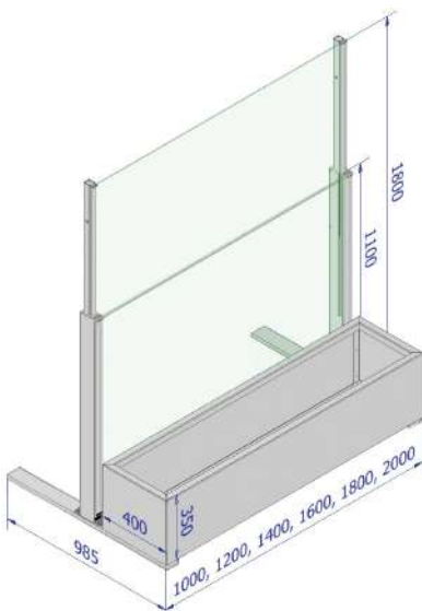
Wind Barrier with aluminium plant pot
